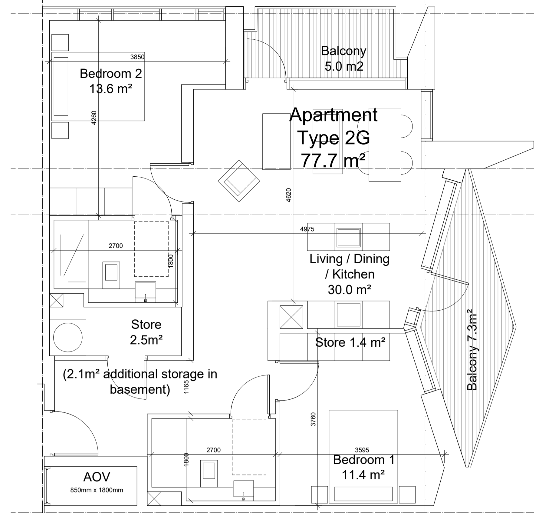
02 PL1924 2 Bed Apartment - Type 2G (10 Units) SCALE 1:50
