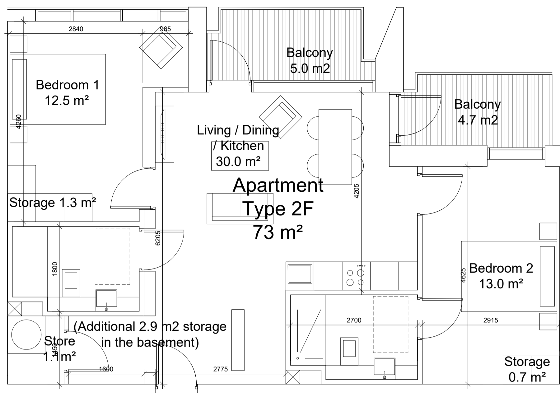
01 PL1924 2 Bed Apartment - Type 2F (2 Units) SCALE 1:50
