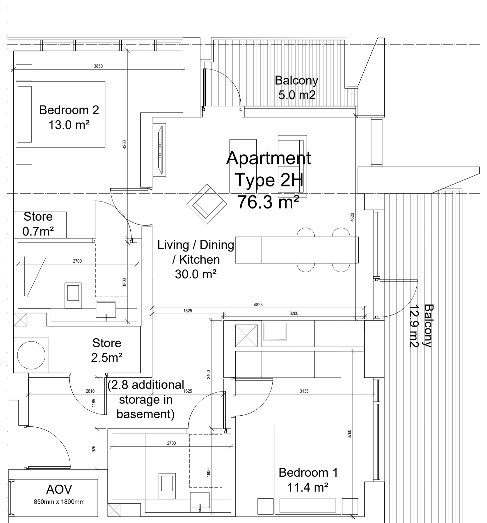
03 PL1924 2 Bed Apartment - Type 2H (2 Units) SCALE 1:50
